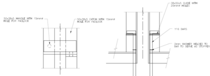
DETAIL C (FRONT ELEVATION)
