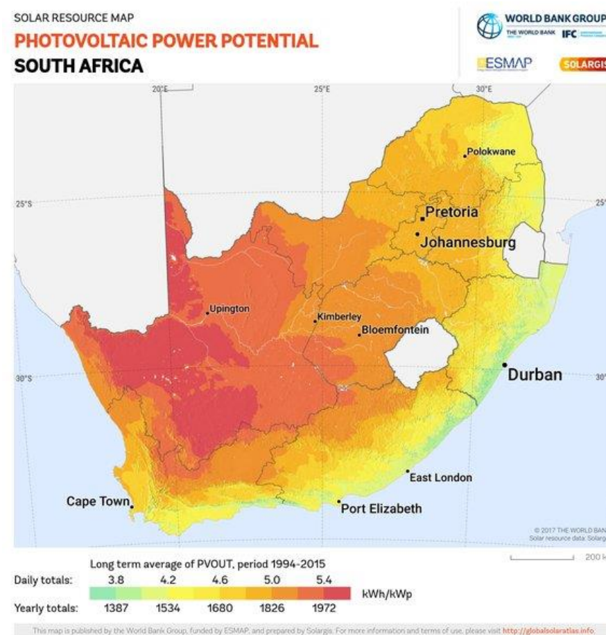
Figure 25: Photovoltaic Power Potential
